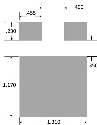
Recommended Stencil Openings
