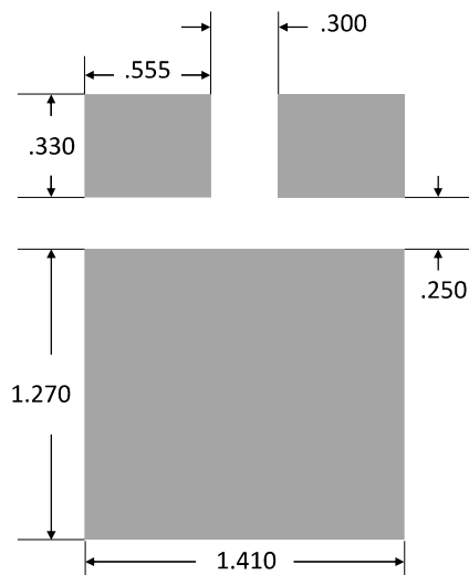
Recommended Solder Pad (Solder Mask Pattern)
