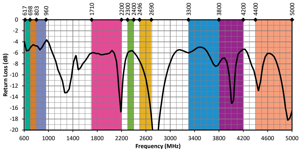
Figure 5. ANT-5GWS4-ccc Return Loss, Edge-Bent
