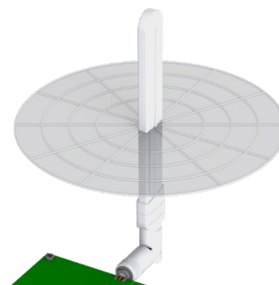
XY-Plane Gain
