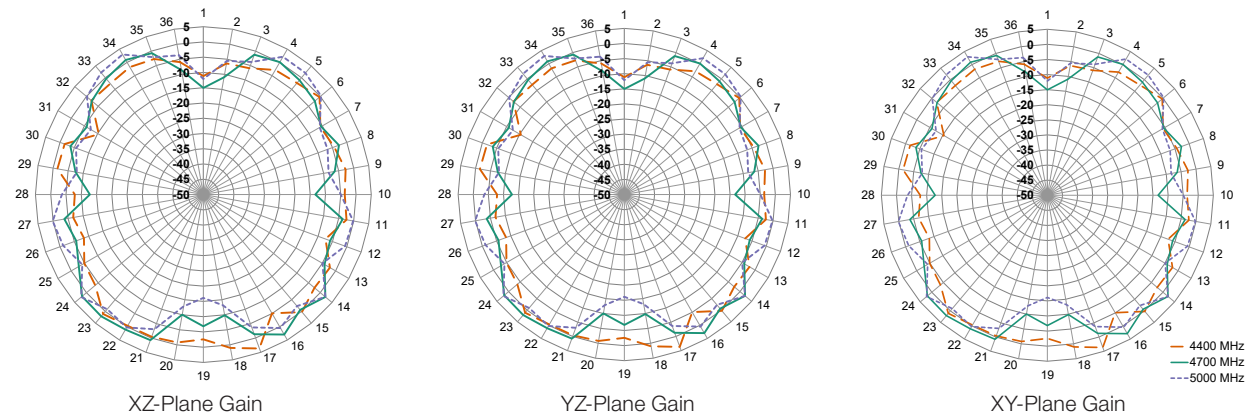
Figure 16. Radiation Patterns for ANT-5GWWS4-ccc, Straight
