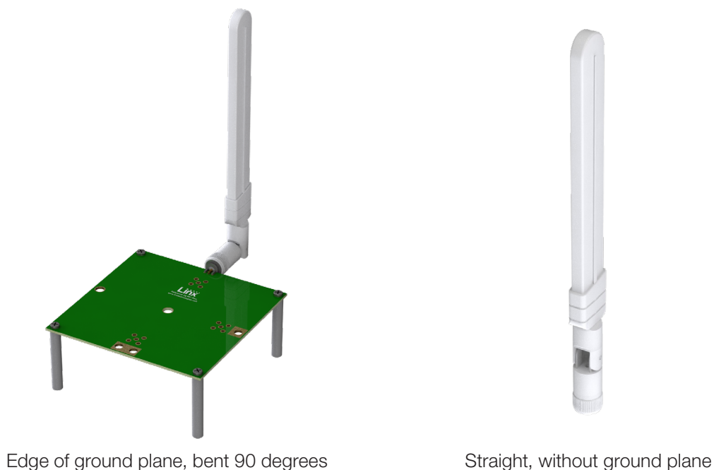
Figure 2. ANT-5GWS4-ccc on evaluation PCB
