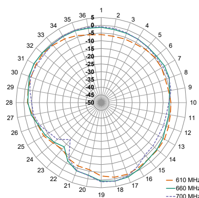
XY-Plane Gain
