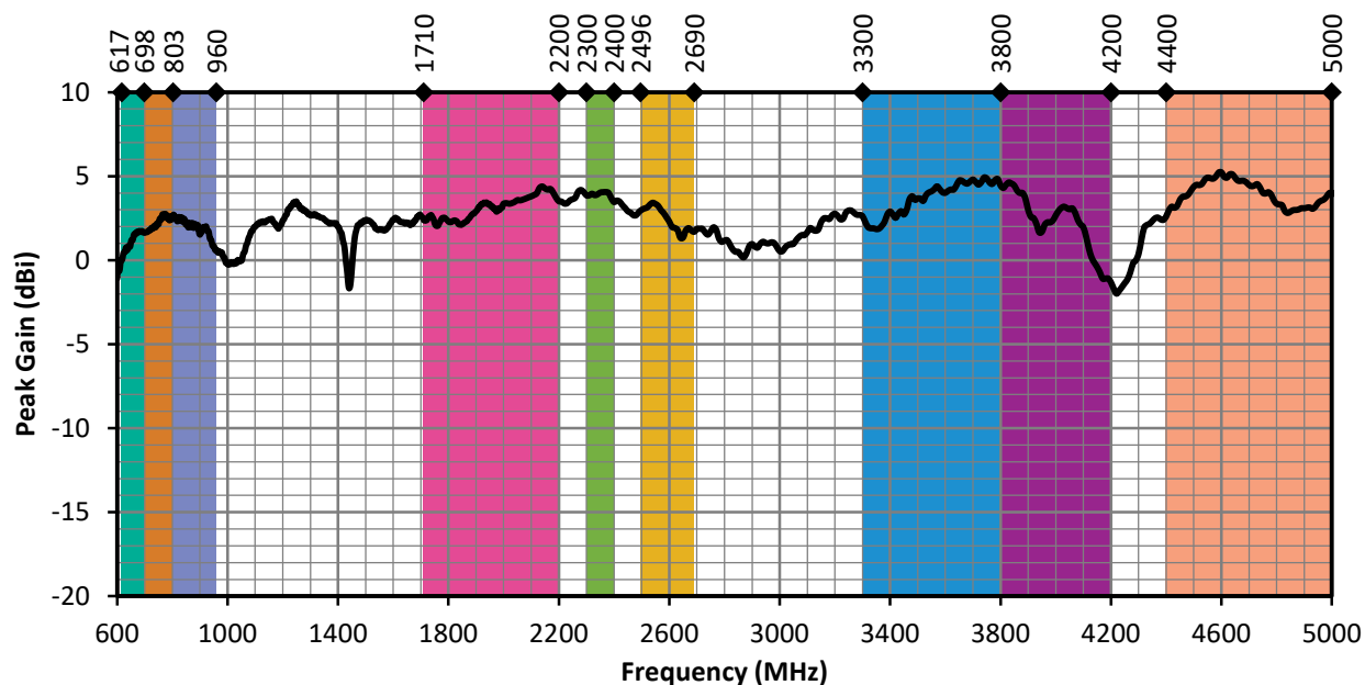
Figure 6. ANT-5GWS4-ccc Peak Gain, Edge-Bent
