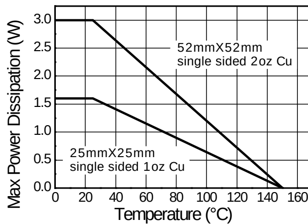
Derating Curve
