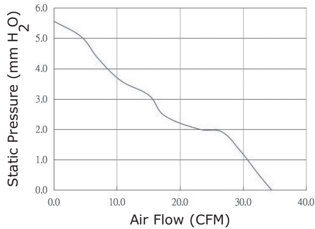
CFM-7025C-240-394
