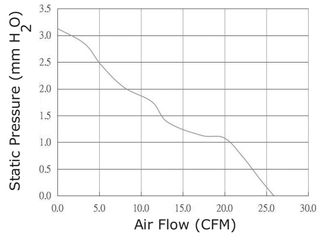
CFM-7025C-230-332
