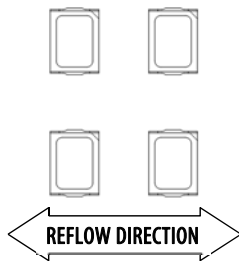
Figure 22: Recommended Board Reflow Direction
