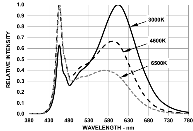
Figure 4: Spectral Power Distribution
