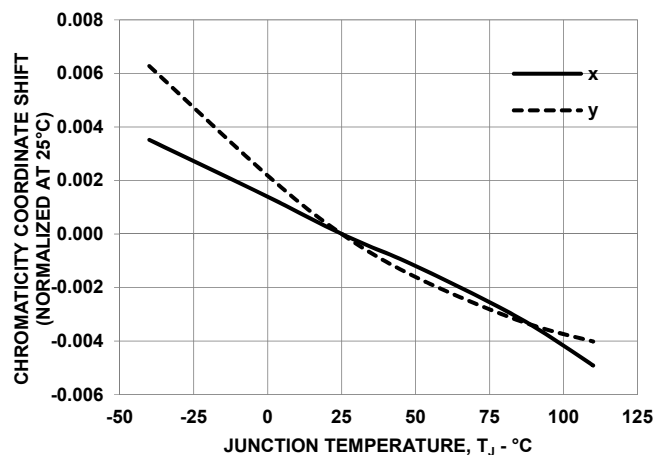
Figure 15: Chromaticity Coordinate Shift vs. Junction Temperature (6500K)
