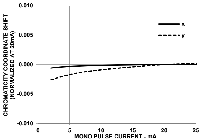
Figure 10: Chromaticity Coordinate Shift vs. Mono Pulse Current (6500K)
