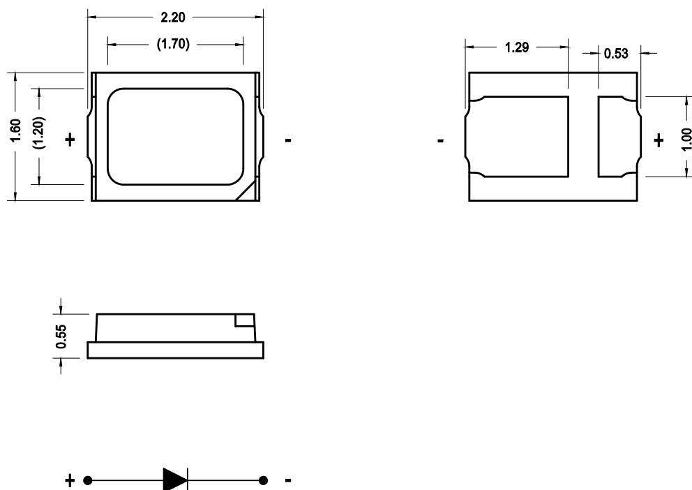
Figure 1: Package Drawing
