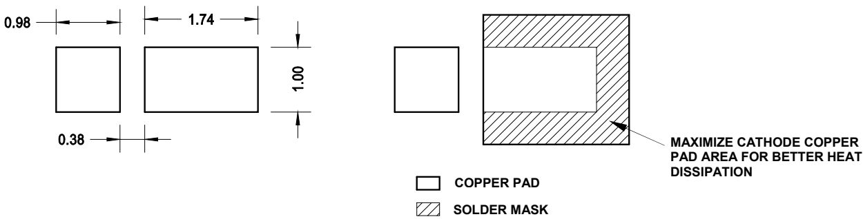
Figure 18: Recommended Soldering Land Pattern
