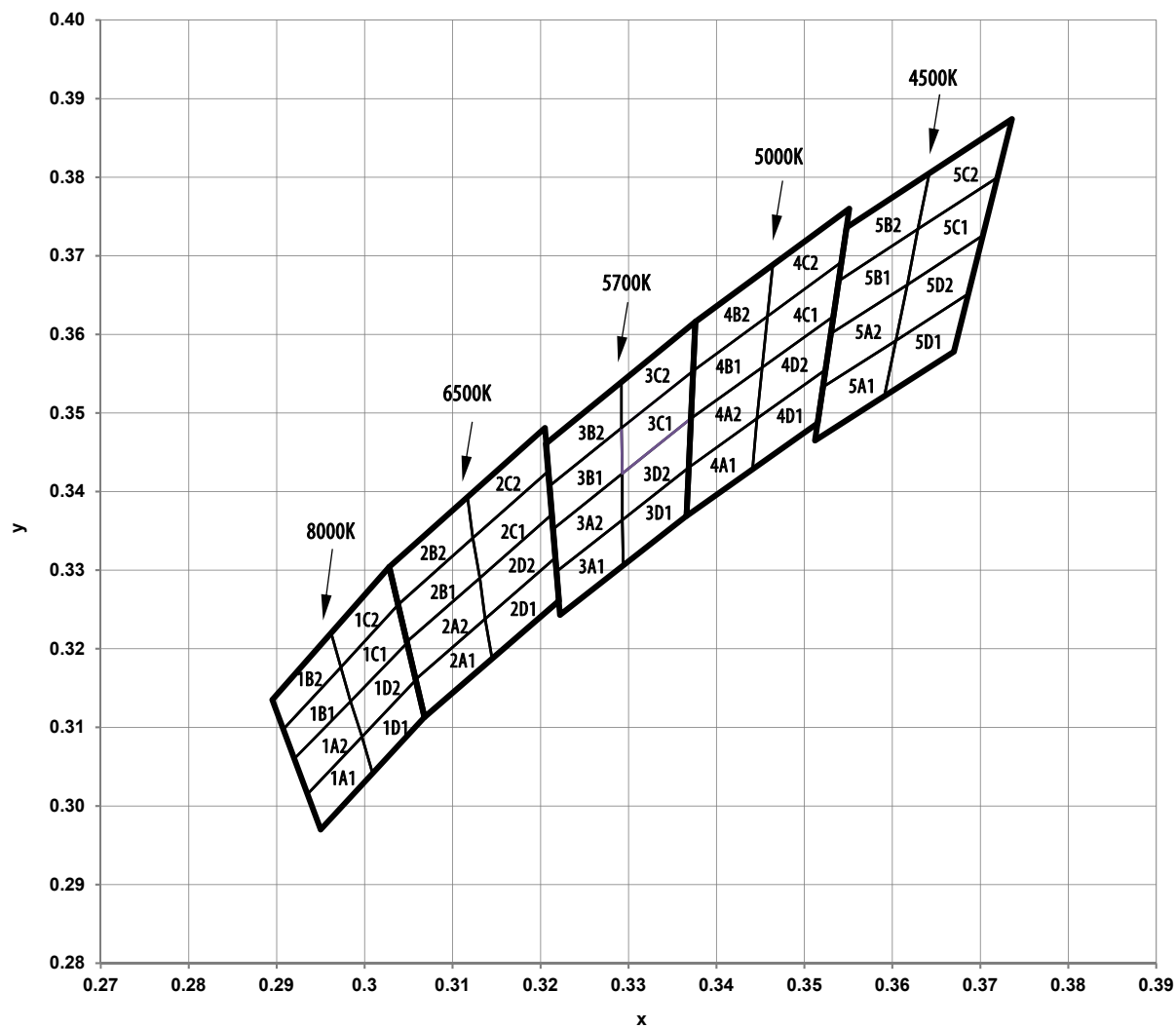
Figure 2: Chromaticity Diagram (4500K-8000K)
