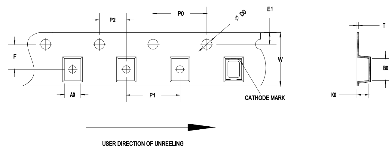
Figure 19: Carrier Tape Dimensions
