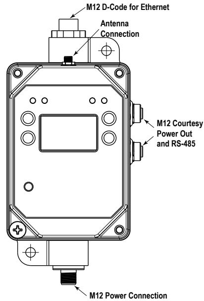
Figure 5. DXM1200E Controller
