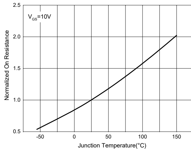
Fig.4 - Normalized On Resistance Characteristics
