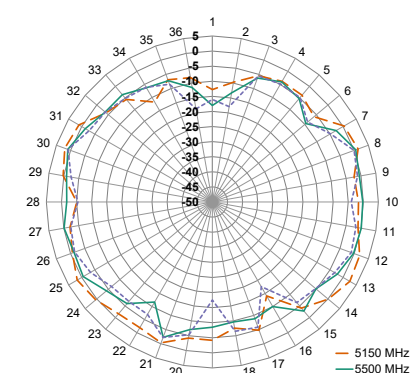
XY-Plane Gain
