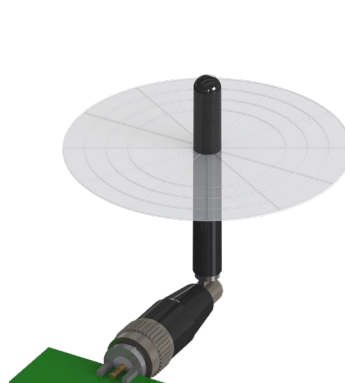
XY-Plane Gain
