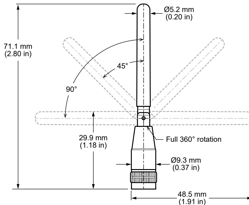
Figure 1. ANT-W63-MON-ccc Antenna Dimensions
