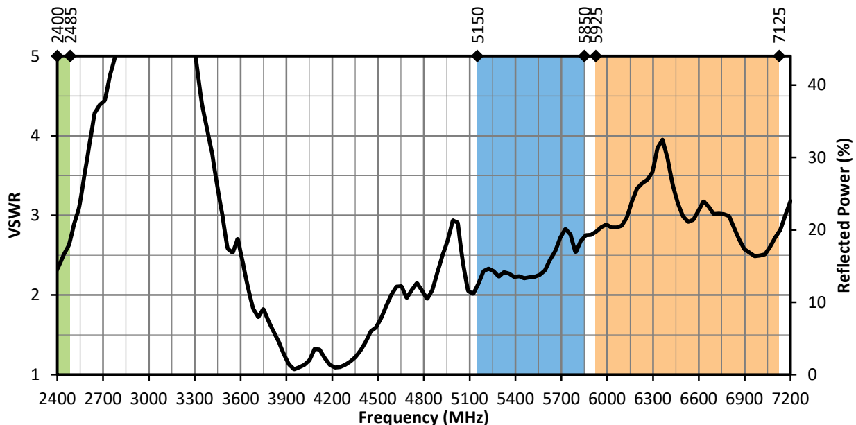
Figure 18. ANT-W63-MON VSWR, Edge-Bent
