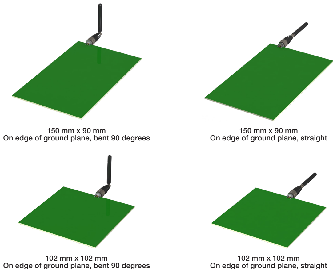
Figure 2. ANT-W63-MON-ccc Test Orientations
