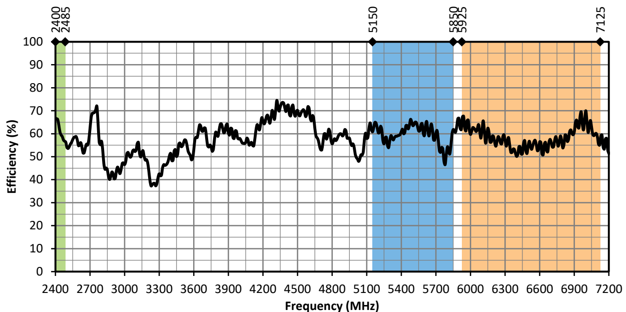
Figure 22. ANT-W63-MON Antenna Efficiency, Edge-Bent
