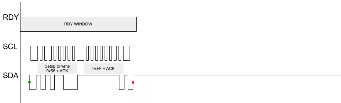
Figure 9.3: Force Stop Communication Sequence
