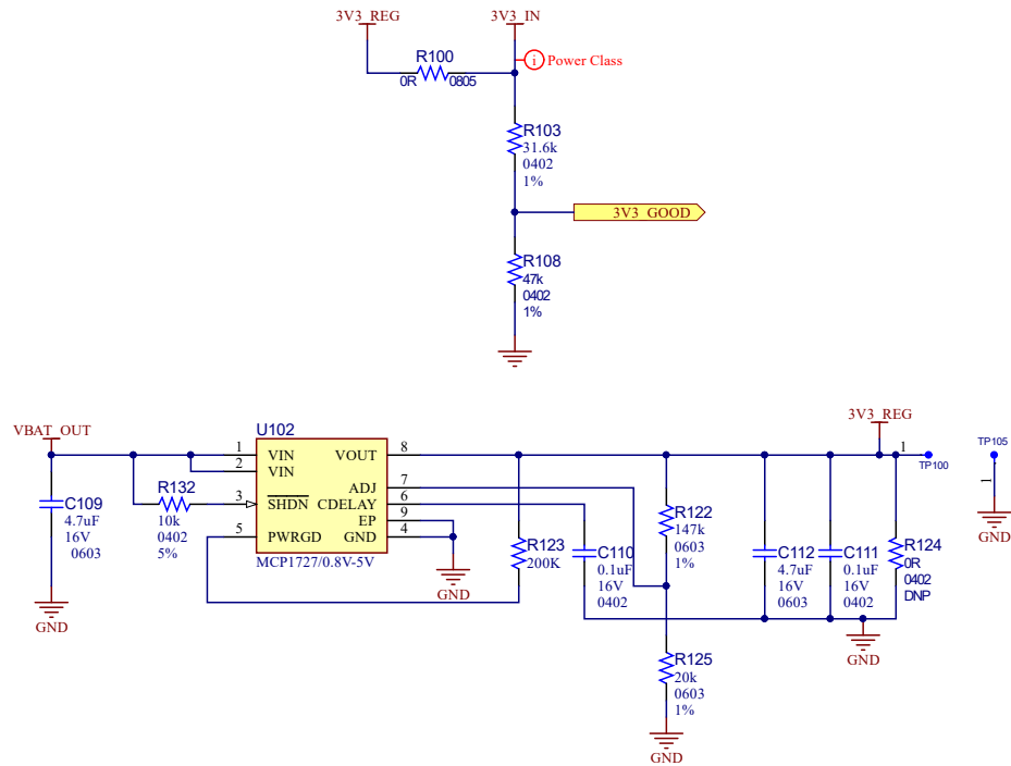
Figure 5-4. 3.3V Regulator for PKOB4
