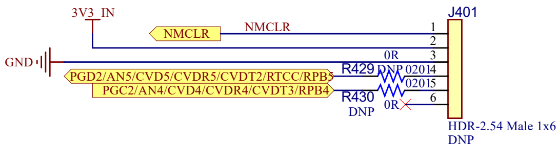
Figure 5-17. ICSP HDR
