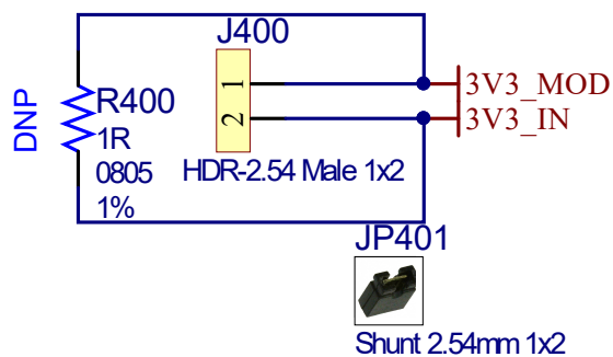
Figure 5-12. TGT Current Measurement Header
