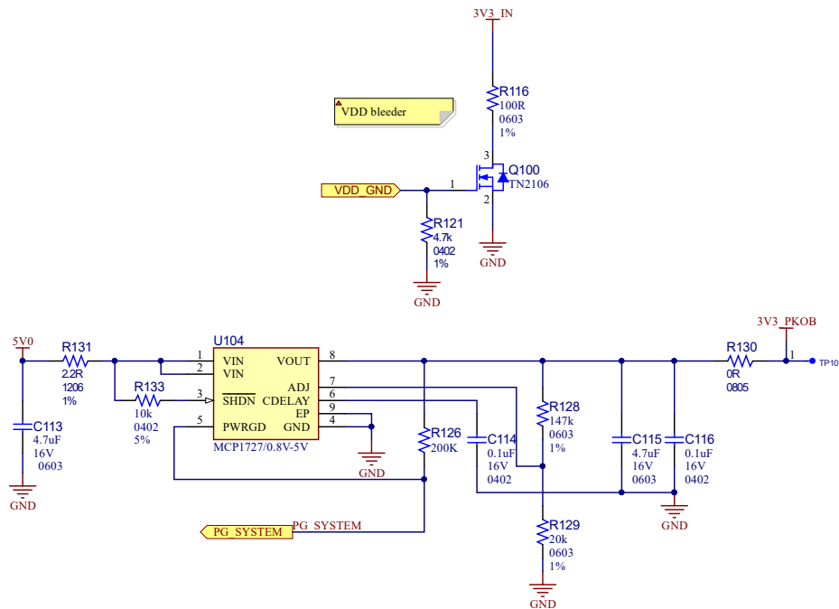
Figure 5-4. 3.3V Regulator for PKOB4
