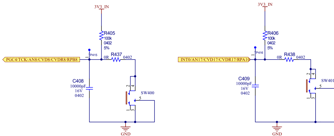
Figure 5-14. Buttons
