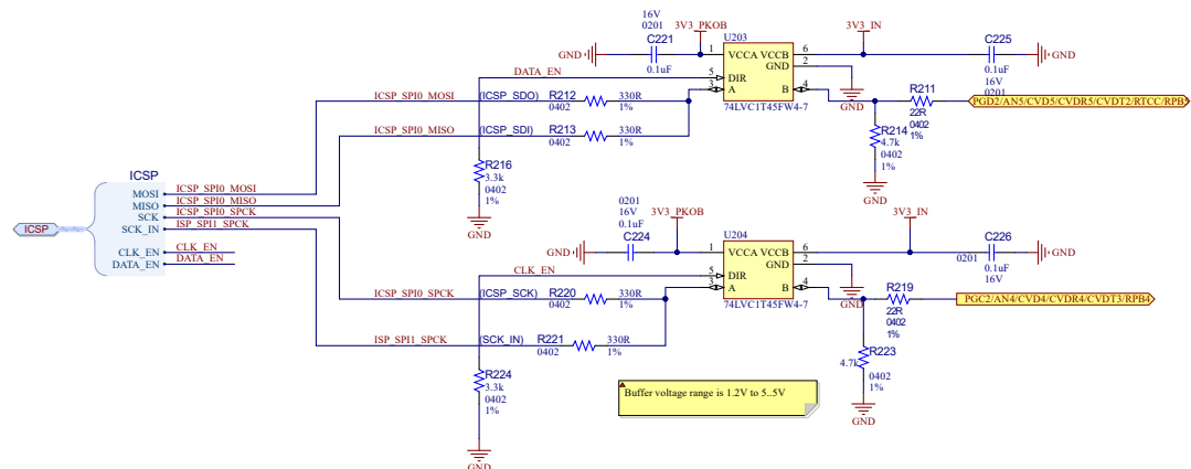
Figure 5-7. ICSP
