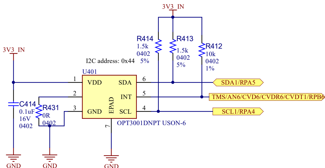
Figure 5-16. Temperature Sensor
