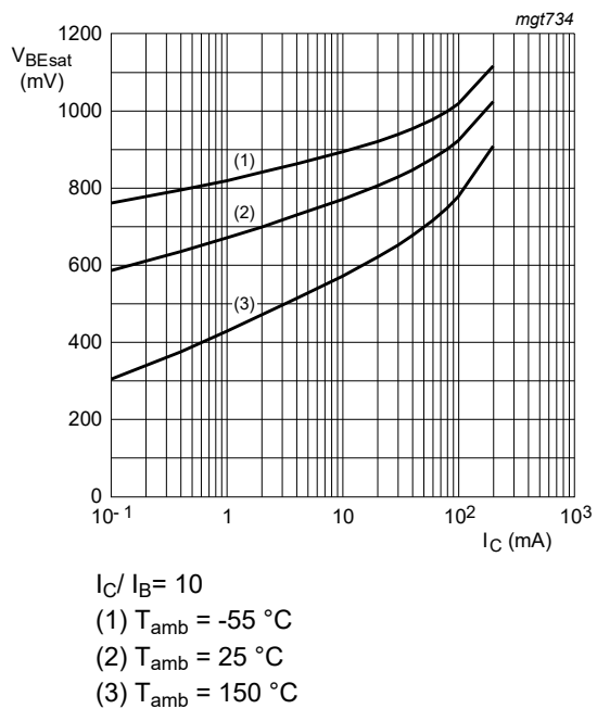
Fig. 15. BC847CQB-Q: Base-emitter saturation voltage as a function of collector current; typical values
