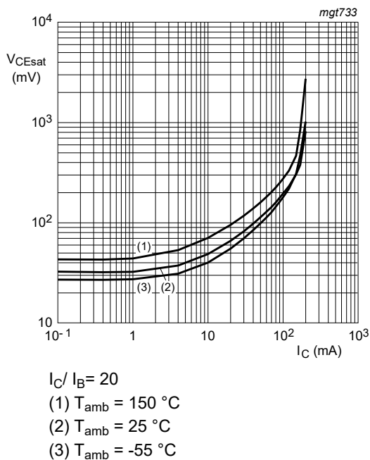
Fig. 14. BC847CQB-Q: Collector-emitter saturation voltage as a function of collector current; typical values
