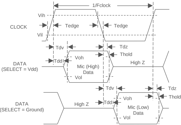
Figure 1: Timing Diagram
