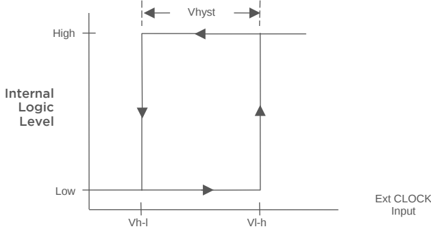
Figure 2: Hysteresis Diagram
