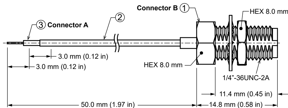
Figure 1. Product Dimensions for the CSS-SGAF-050-STTN Cable Assembly
