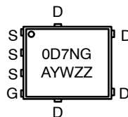
DFN5 (SO-8FL) CASE 506EZ
