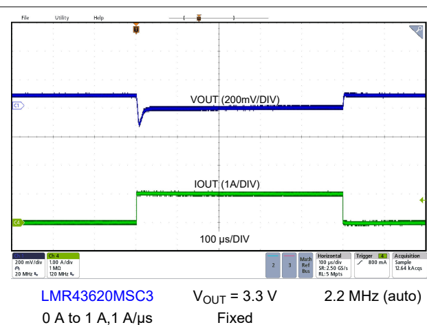
Figure 9-18. Load Transient
