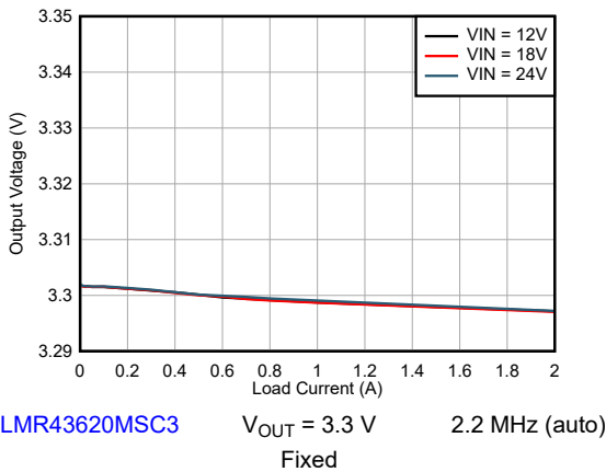
Figure 9-11. Line and Load Regulation
