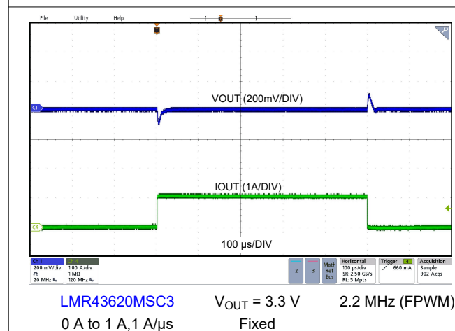
Figure 9-17. Load Transient
