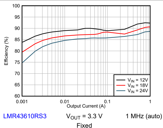
Figure 9-7. Efficiency
