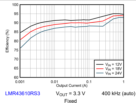
Figure 9-8. Efficiency
