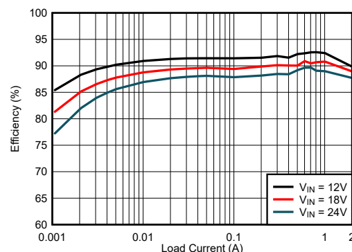
Efficiency: V_{OUT} = 3.3 \text{ V} (Fixed), 2.2 MHz
