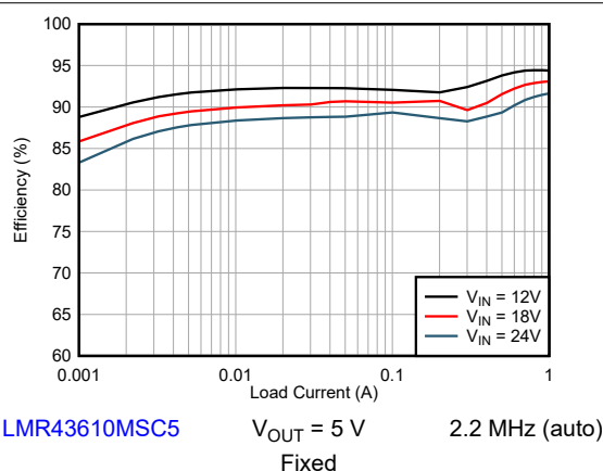
Figure 9-5. Efficiency
