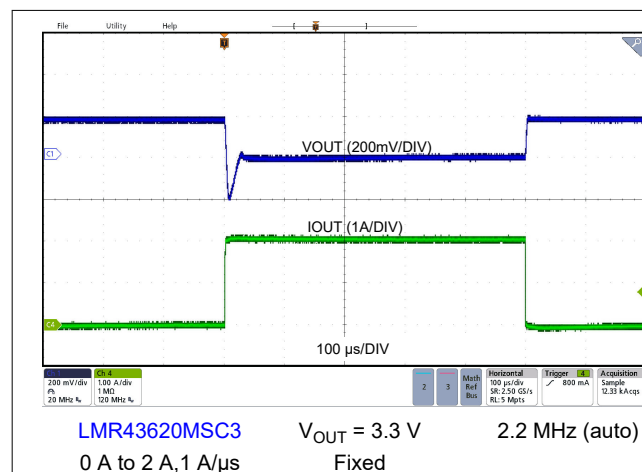
Figure 9-15. Load Transient
