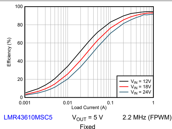
Figure 9-6. Efficiency
