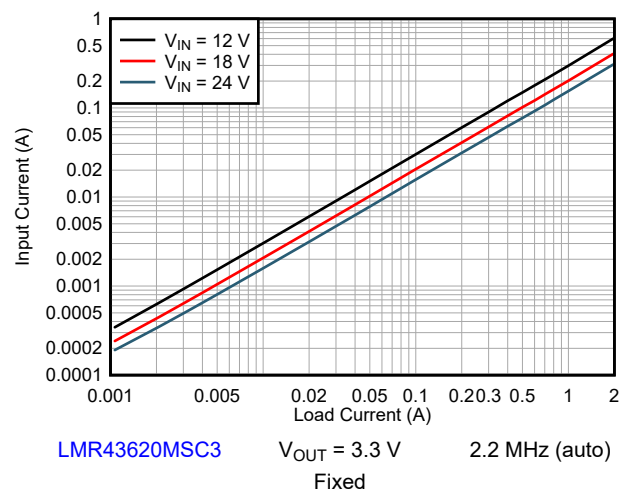
Figure 9-14. Input Current vs. Load Current
