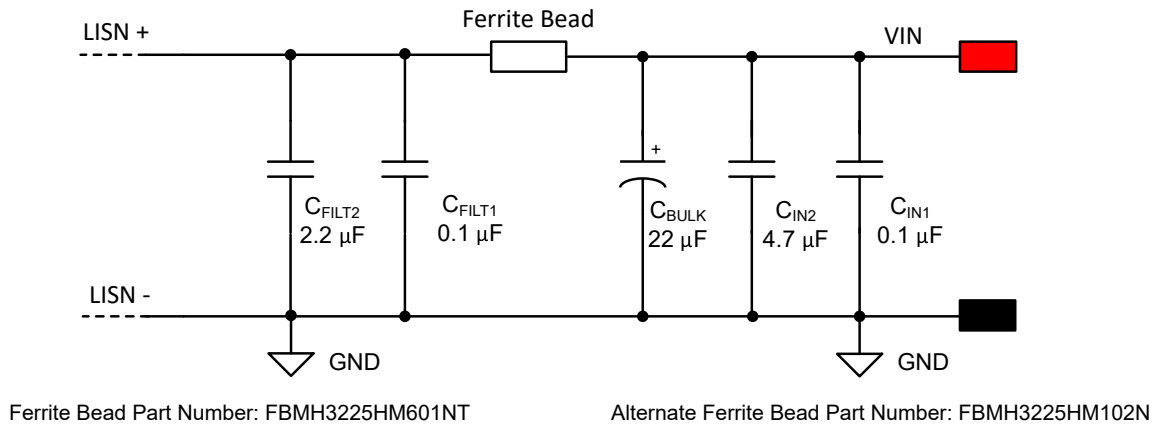
Figure 9-29. Typical Input EMI Filter
