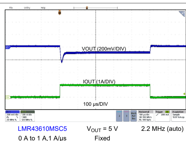
Figure 9-20. Load Transient
