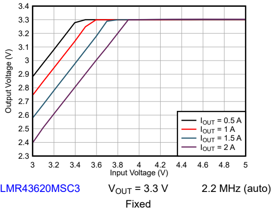
Figure 9-9. Dropout
