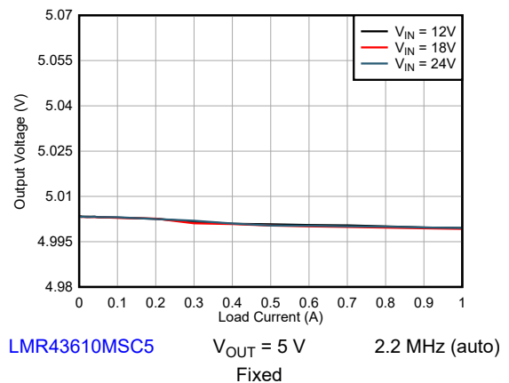
Figure 9-12. Line and Load Regulation
