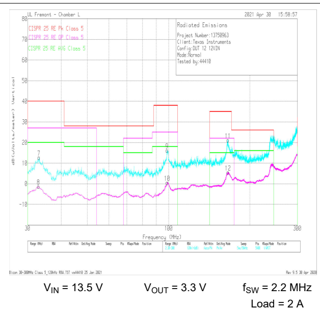
Figure 9-28. Typical CISPR 25 Radiated EMI 30 MHz–300 MHz Vertical Bicon Antenna Blue: Peak Detect, Pink = Average Detect
