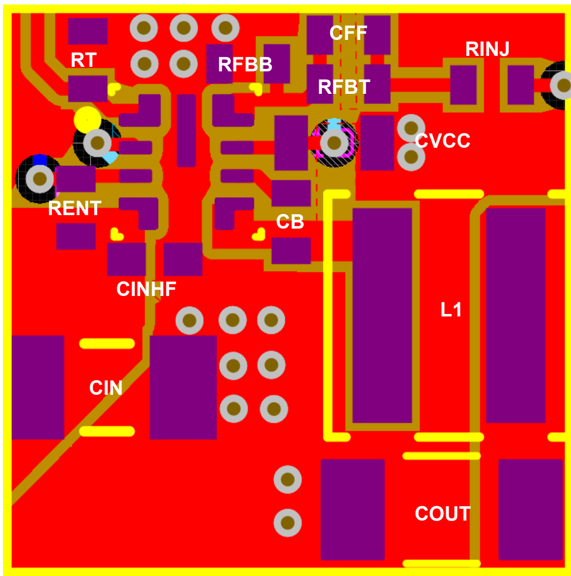
Figure 11-2. Example Layout
