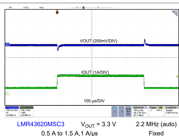
Figure 9-16. Load Transient
