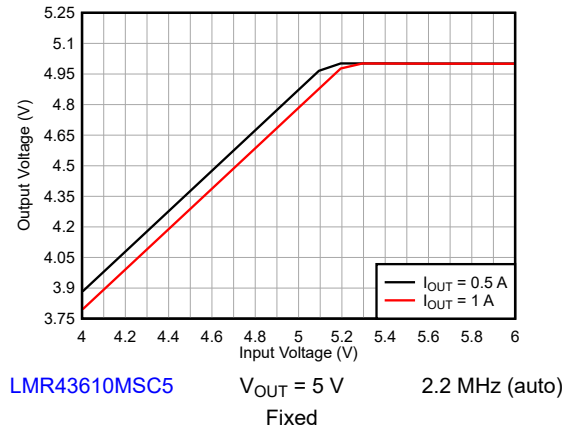
Figure 9-10. Dropout
