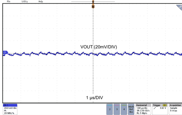
LMR43620MSC3 V_{OUT} = 3.3\text{ V} 2-A load Fixed
