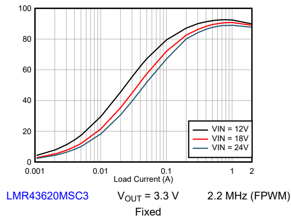
Figure 9-4. Efficiency
