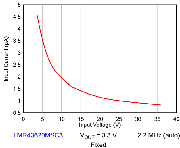
Figure 9-13. Input Switching Current vs. Input Voltage
