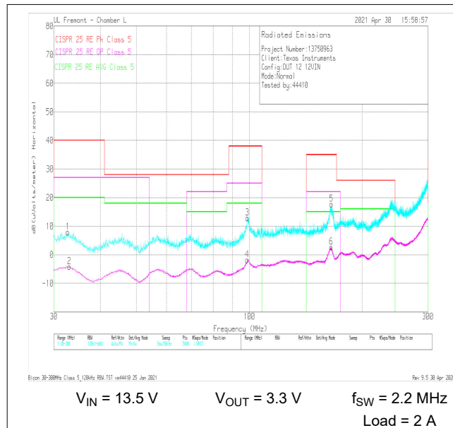
Figure 9-27. Typical CISPR 25 Radiated EMI 30 MHz–300 MHz Horizontal Bicon Antenna Blue: Peak Detect, Pink = Average Detect
