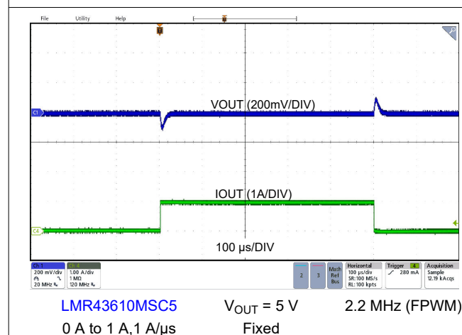
Figure 9-19. Load Transient
