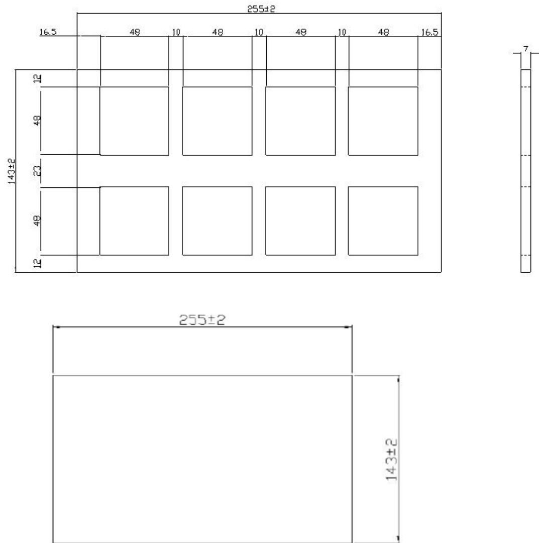
Splitter Plate Drawing (EVA material)
