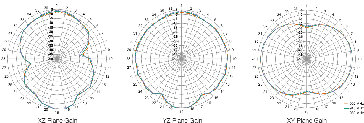
Figure 9. Radiation Patterns for ANT-8/9-PW-LPN Antenna, Edge of ground Plane
