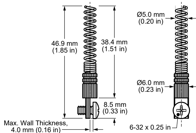
Figure 1. ANT-8/9-PW-LPN Antenna Dimensions
