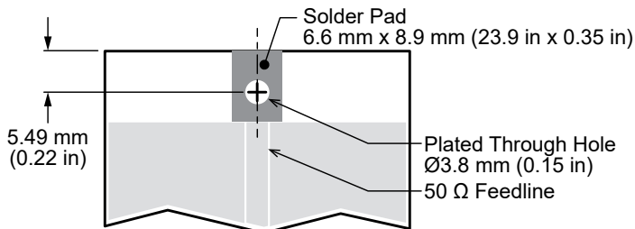
Figure 2. ANT-8/9-PW-LPN Recommended Mounting and PCB Footprint
