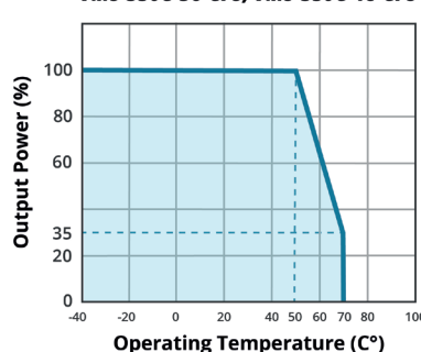
TEMPERATURE DERATING CURVE (full load 550W with 25 CFM) VMS-550C-24-CFS, VMS-550C-27-CFS VMS-550C-36-CFS, VMS-550C-48-CFS
