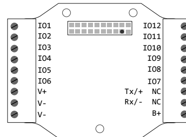
Figure 3. P7C model wiring board
