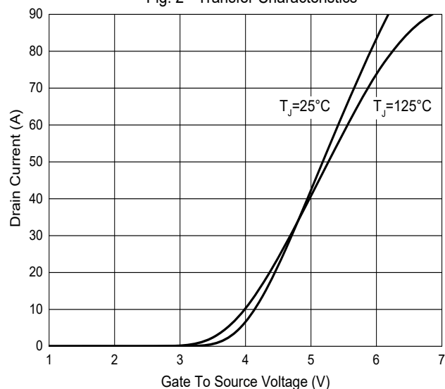
Fig. 2 - Transfer Characteristics
