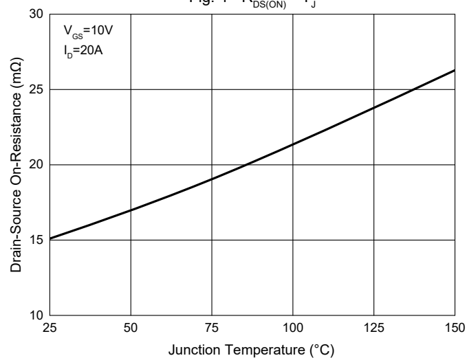
Fig. 4 - R_{DS(ON)} - T_J
