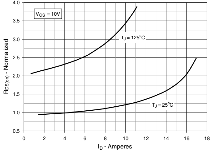
Fig. 5. R_{DS(on)} Normalized to I_D = 4A Value vs. Drain Current
