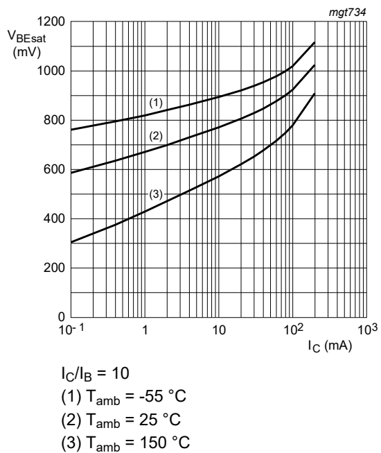
Fig. 13. BC847CW-Q: Base-emitter saturation voltage as a function of collector current; typical values
