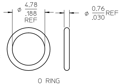
O RING
