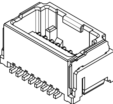
16-24極 16-24 CIRCUIT
