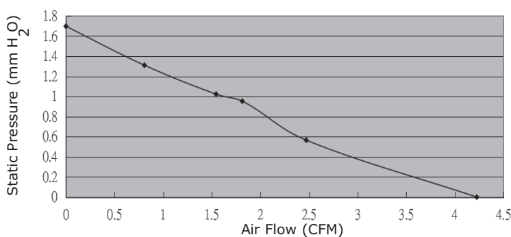
CFM-4010C-150-195
