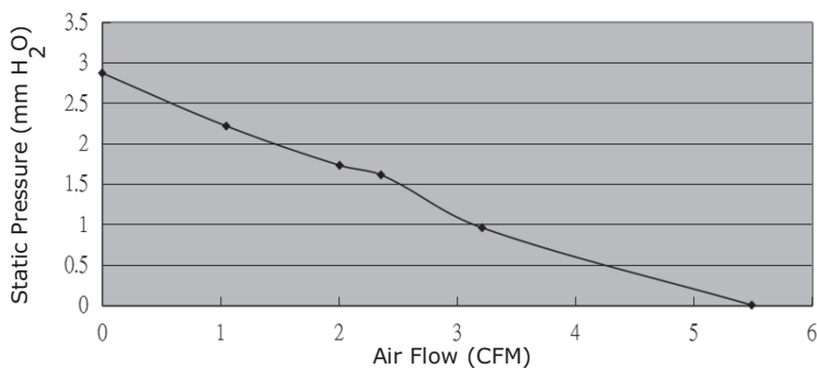
CFM-4010C-065-251
