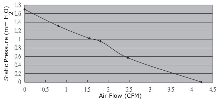
CFM-4010C-250-195
