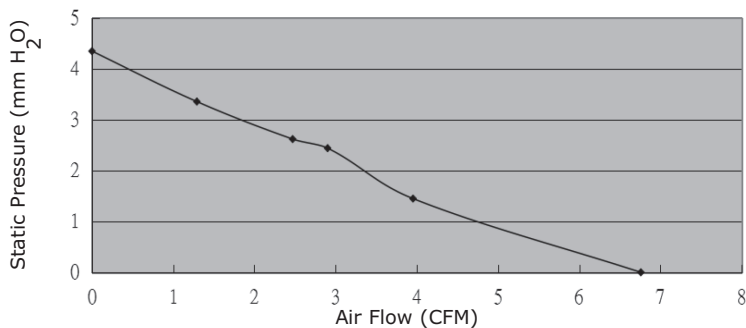
CFM-4010C-180-296
