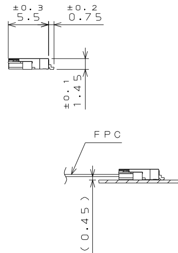
MATED CONDITION (REF.) 嵌合状態図 (参考)
