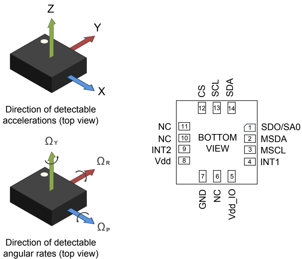
Figure 4. Pin connections
