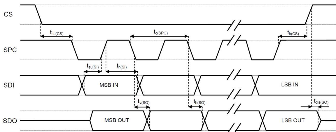
Figure 6. SPI slave timing diagram (in mode 3)
