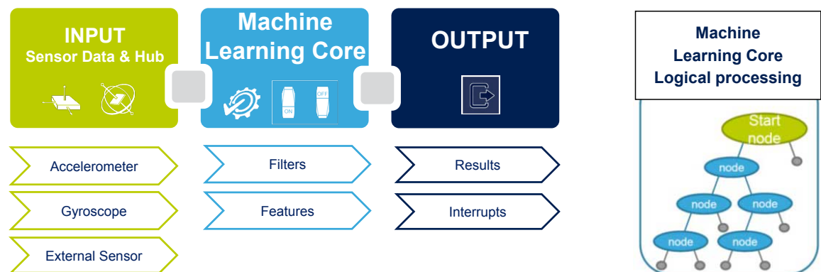
Figure 3. Machine learning core in the ASM330LHHX
