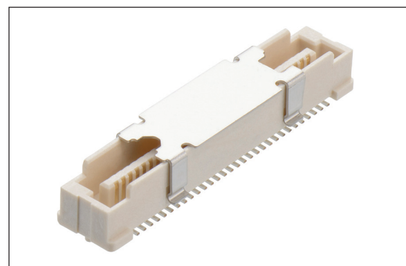
60 contact (30+30) male Archer .8 with pick and place cap assembled
