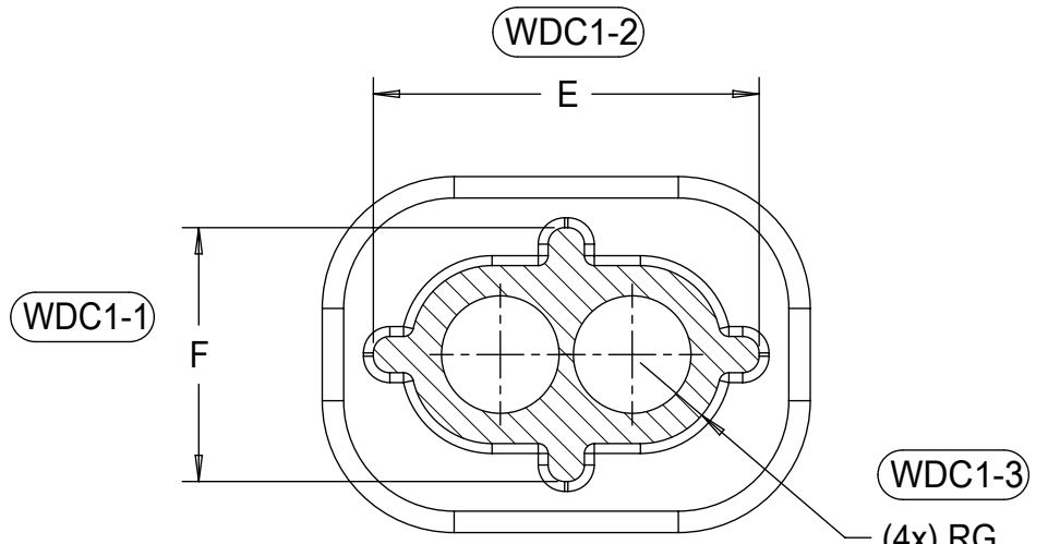
SECTION Z-Z
