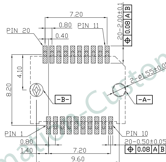
RECOMMENDED PCB LAYOUT(TOP VIEW) (ALL TOLERANCES ARE ±0.05)
