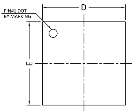
Package Dimensions, QFN5x5-31L
