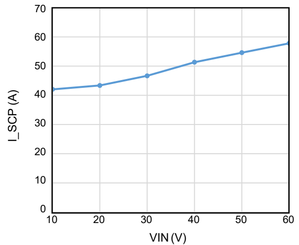
Figure 3. I_{SCP} vs. VIN, Short Current Protection Curve
