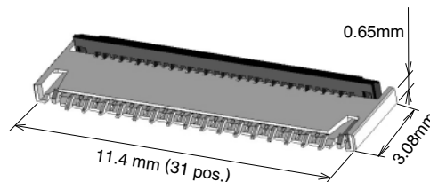
0.65mm height
