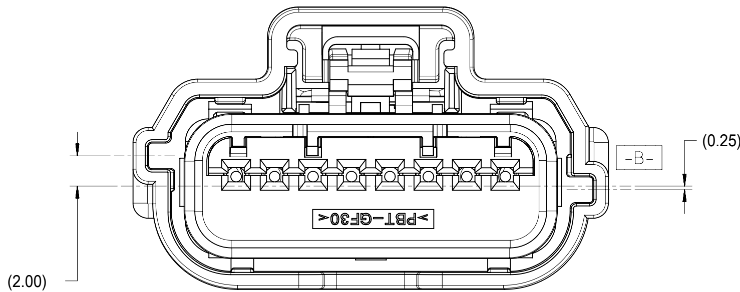
POLARIZATION C
