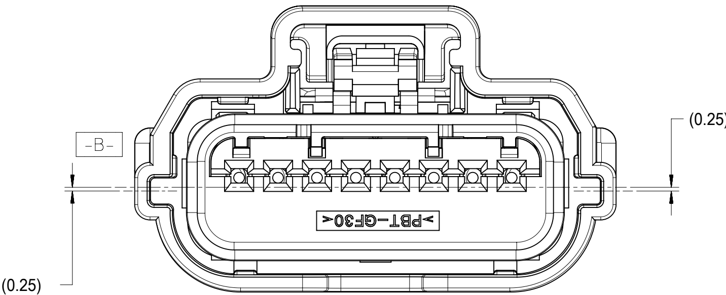
POLARIZATION D
