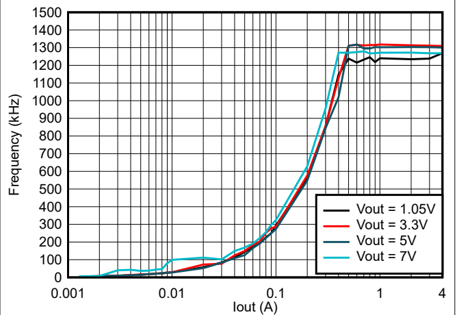
Figure 6-10. TPS564242 Frequency vs Loading
