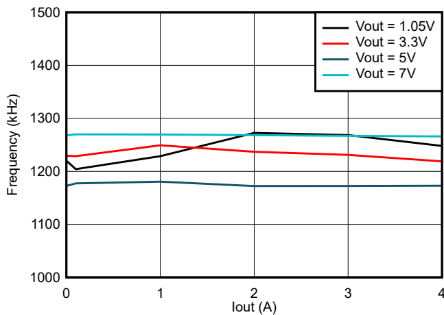
Figure 6-9. TPS564247 Frequency vs Loading
