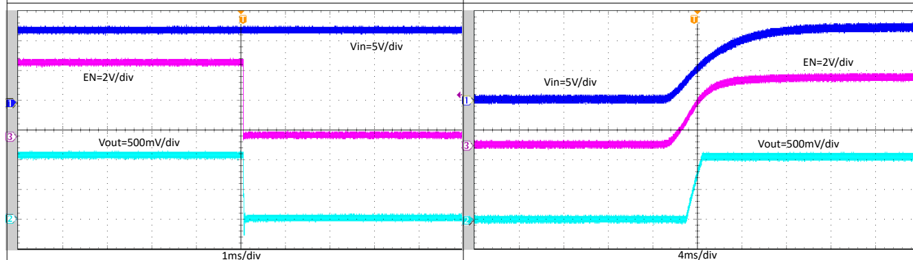
Figure 8-12. Shutdown Through EN, I_{OUT} = 4\text{ A}
