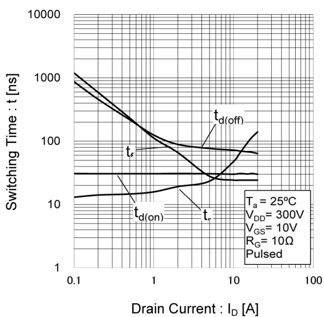
Fig.15 Switching Characteristics
