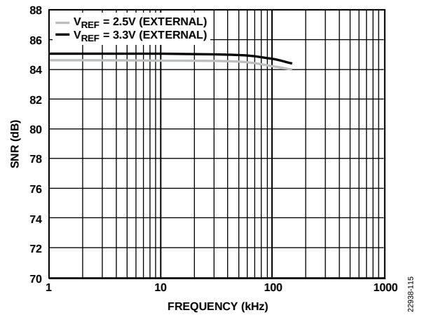
Figure 15. SNR vs. Frequency
