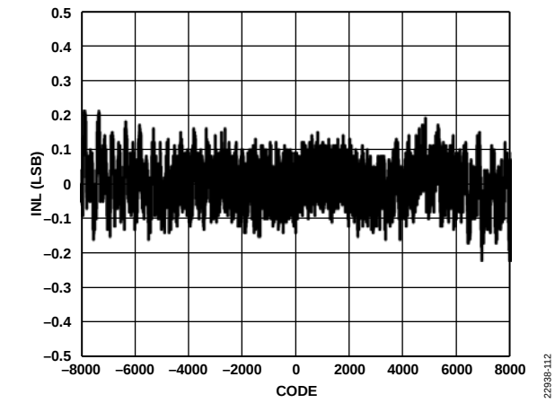
Figure 12. INL vs. Code
