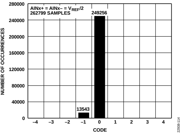
Figure 14. Code Histogram
