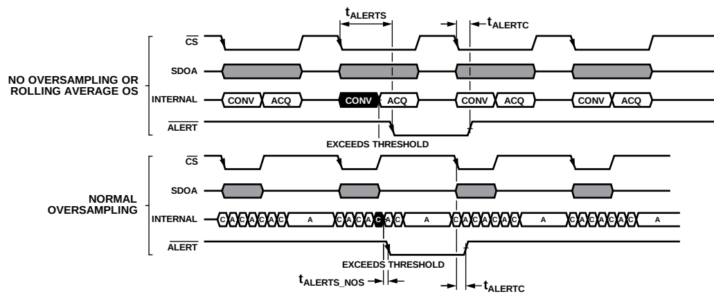
Figure 8. ALERT Timing
