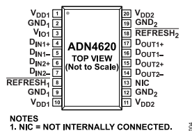
Figure 5. ADN4620 Pin Configuration, SSOP
