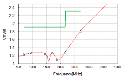
Lo-Band Port VSWR
