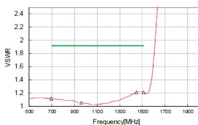
Lo-Band Port VSWR
