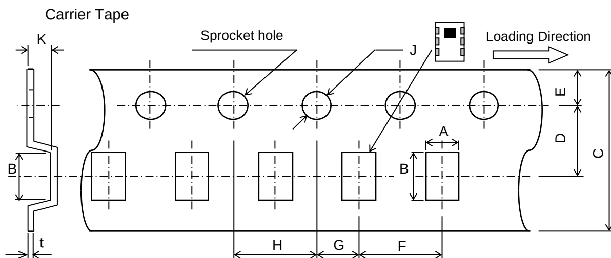
Dimensions (mm)
