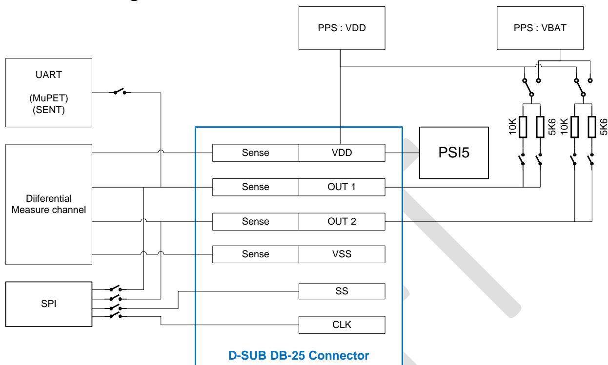
Figure 2: Functional diagram
