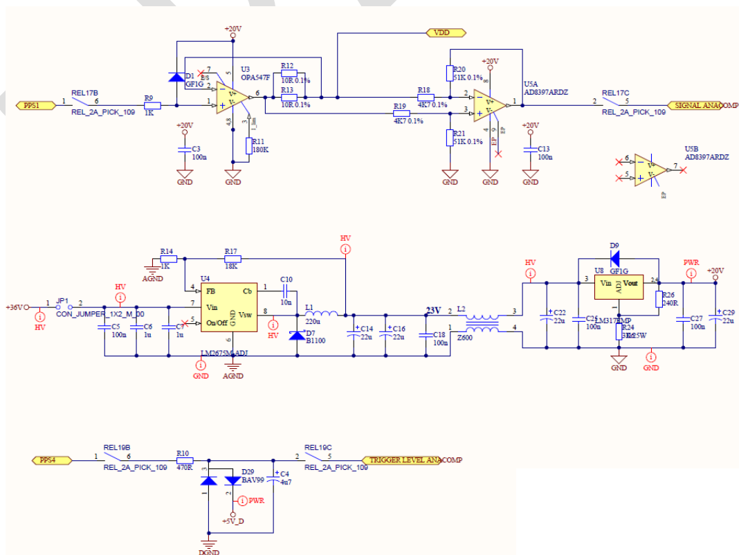
Figure 11: PS15 Block
