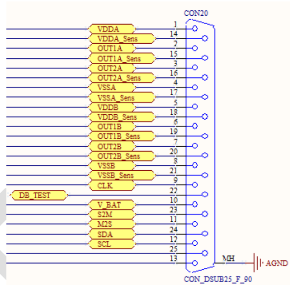
Figure 14: DB-25 device connector.
