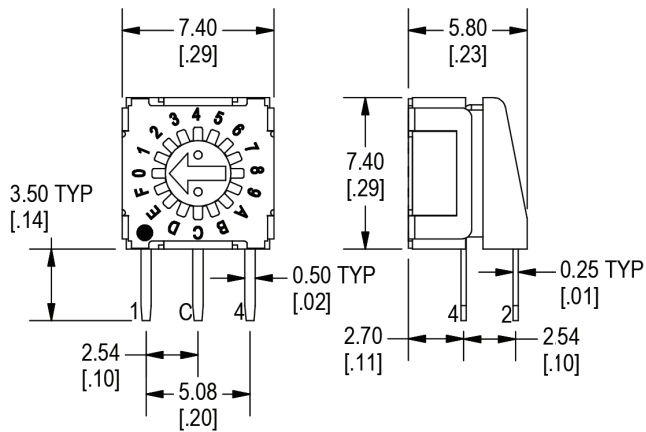
T Terminals
