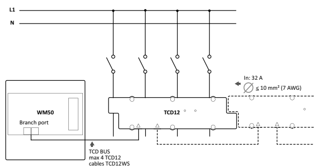
Fig. 12 Single-phase system with neutral (2-wire)
